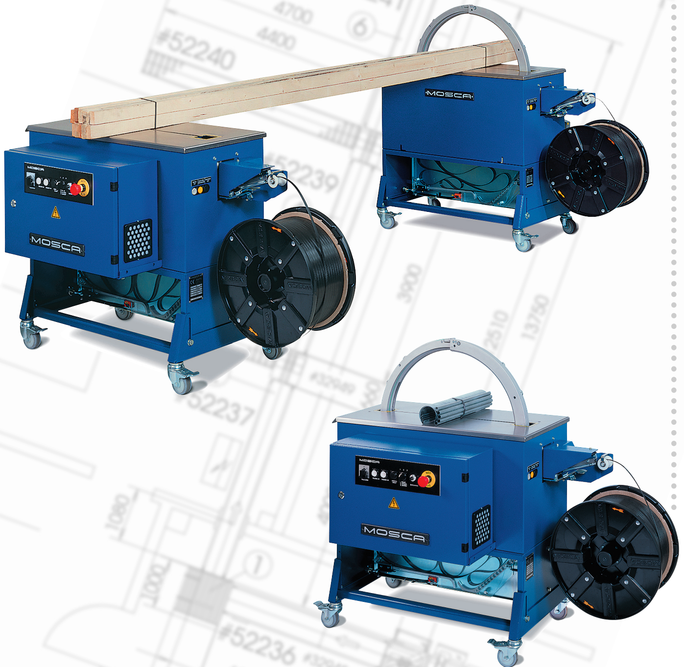
RO-M-RI STRAPPING MACHINE WITH RING-SHAPED STRAP FEED ARCH
